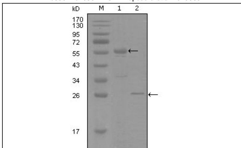
Figure 1: Western blot analysis using PGR mouse mAb against truncated MBP-PGR recombinant protein (1) and truncated Trx-PGR(aa730-871) recombinant protein (2).
