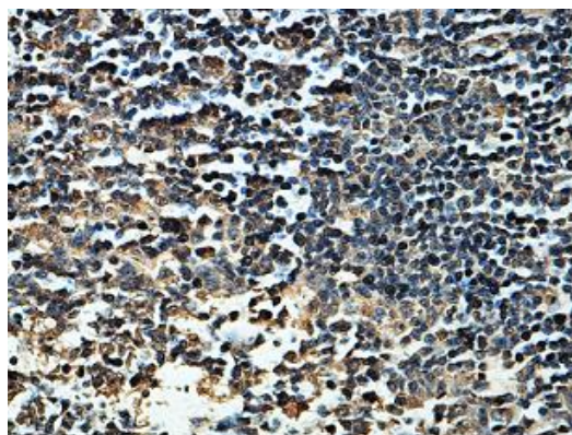
Immunohistochemical staining of formalin-fixed paraffin-embedded tonsil showing membrane staining with anti-CD8 antibody at a dilution of 1/100.
