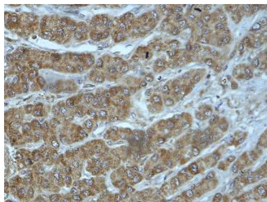
Immunohistochemical staining of formalin-fixed paraffin-embedded liver cancer staining with anti-PPBP antibody at a dilution of 1/100
