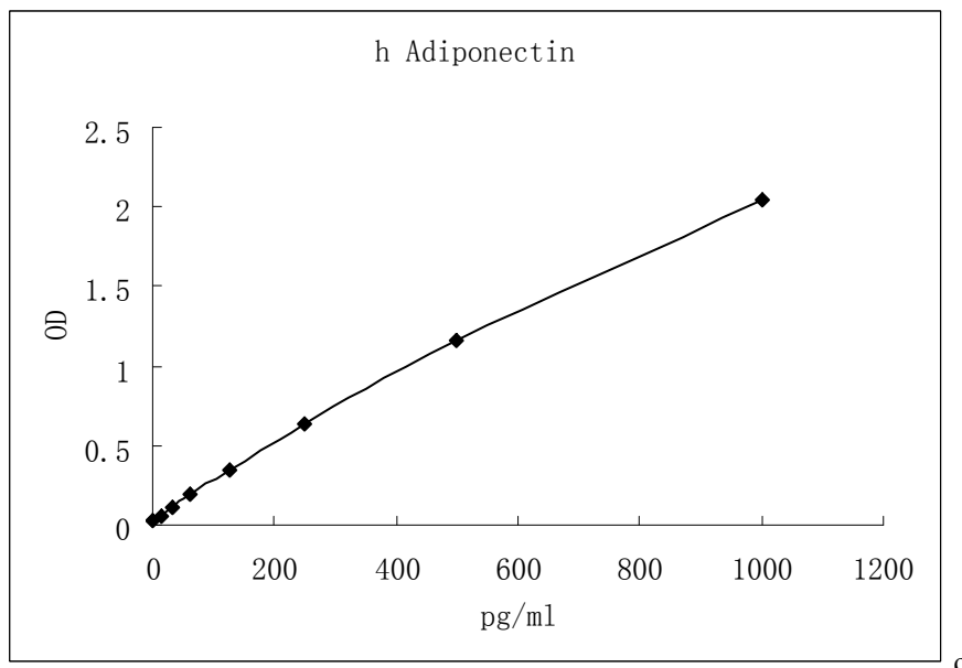
Figure 4: Representative standard curve for Adiponectin ELISA. Adiponectin was diluted in serial two-fold steps in Sample Diluent.
