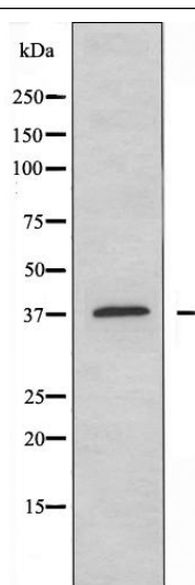
Western blot analysis of extracts from Jurkat cells, using PARD6B antibody.
