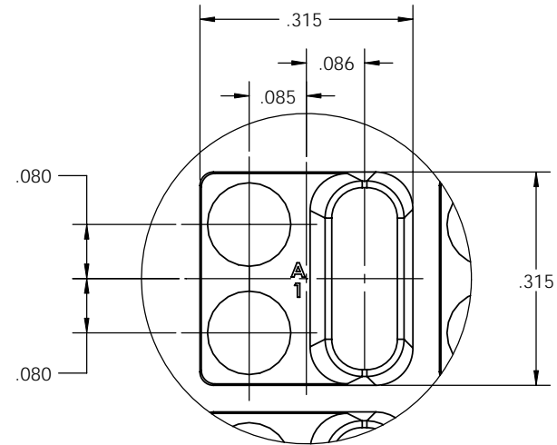
DETAIL A SCALE 6 : 1 96X
