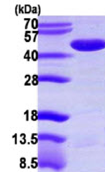
15% SDS-PAGE (3ug)
