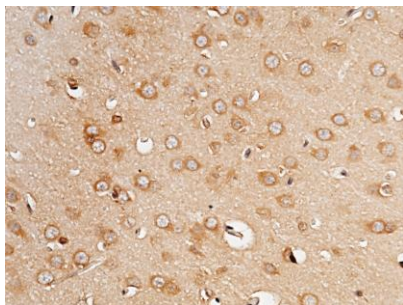
Immunohistochemical staining of rat PCSK9 in rat brain with mouse monoclonal antibody (1:60, formalin-fixed paraffin embedded sections).
