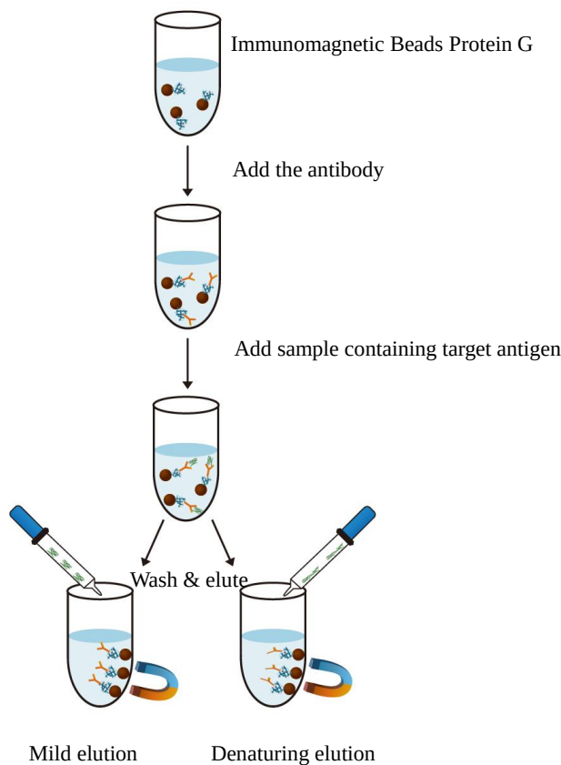
Fig. 1 Immunoprecipitation (IP) Protocol
