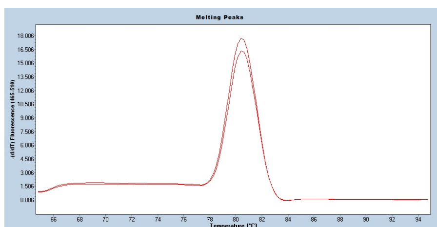
dissolution curves
